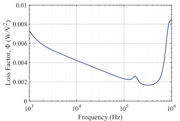
FIGURE 7. The derived loss factor \tilde{\gamma}(\omega) versus frequency.
